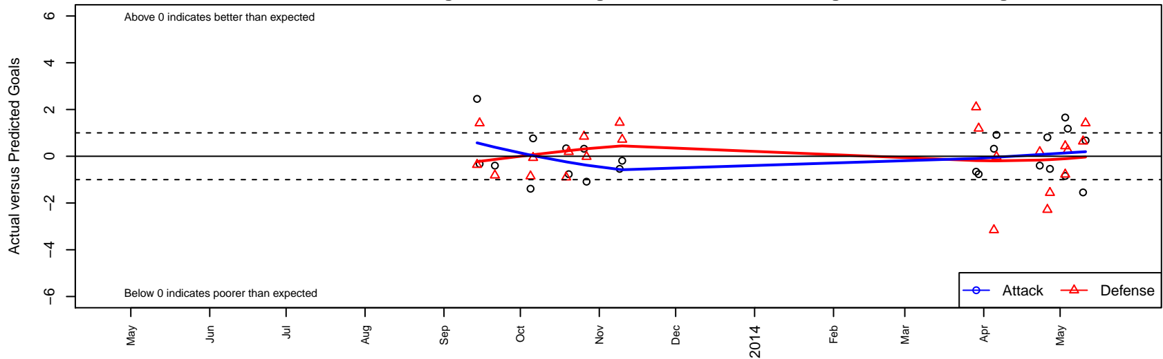
Scorpions SC ECNL G99 Dots are actual minus expected GF (blue circles) and GA (red triangles). Blue line is smoothed change in attack strength. Red is smoothed change in defense strength.
